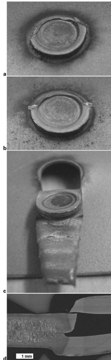
a static; b intermediate; c impact; d fracture cross-section 14 Typical fractured coupon appearance for 590R material
