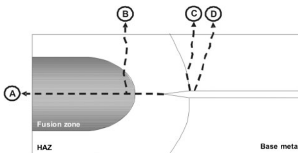
8 Schematic of weld joint cross-section with typical tensile shear failure modes
